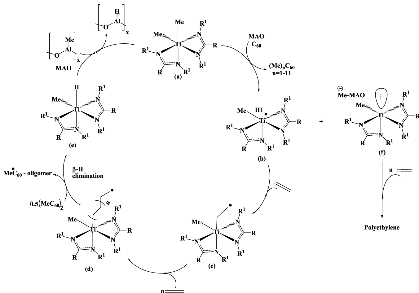
Scheme 4. Plausible Mechanism for Polymerization of Ethylene Catalyzed by a Titanium(IV) Complex
