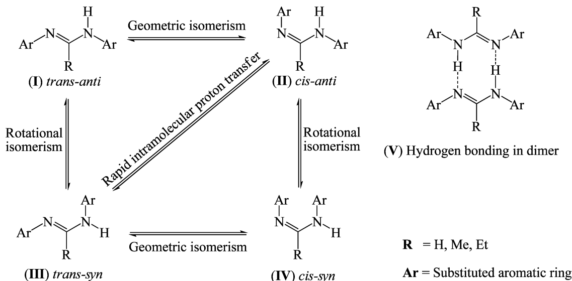
Scheme 2. Plausible Tautomeric Structures for Amidines in Solution
