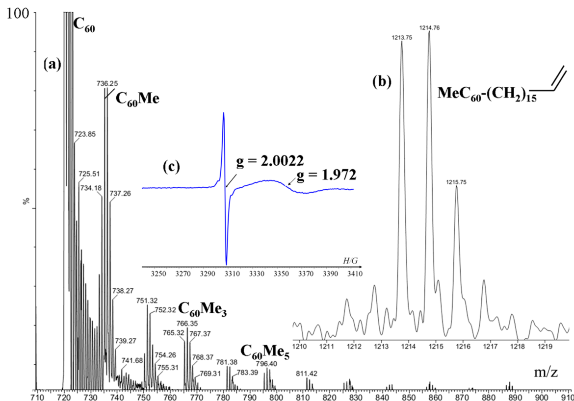
Figure 8. MALDI-TOF analysis of sample prepared from complex 15 and MAO using fullerene as radical trapping agent after backfilling with ethylene. Catalyst added in a ratio of complex 15 :MAO 3:100. (a) MALDI-TOF spectrum of the solid part of the catalytic slurry. (b) Enlargement of the signal that corresponds to the highest mass. (c) ESR spectrum of the reaction mixture.
