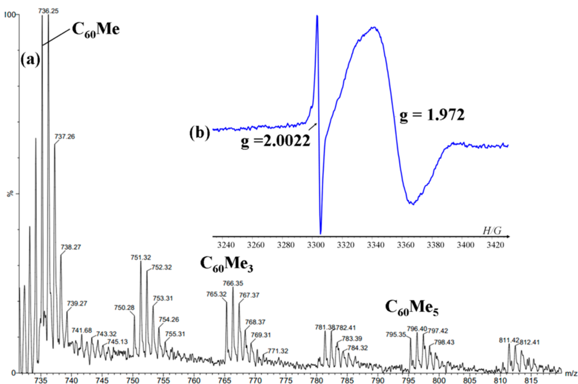
Figure 7. MALDI-TOF analysis of sample prepared from complex 15 and MAO using fullerene as radical trapping agent after backfilling with ethylene. Catalyst added in a ratio of complex 15 :MAO 1:100. (a) MALDI-TOF spectrum of the solid part of catalytic slurry. (b) ESR spectrum of the reaction mixture shows stable adduct of multiple additions of Me-radical to C_{60} ( g = 2.0022 ) and paramagnetic agglomerate of Ti(III) and MAO ( g = 1.972 ).
