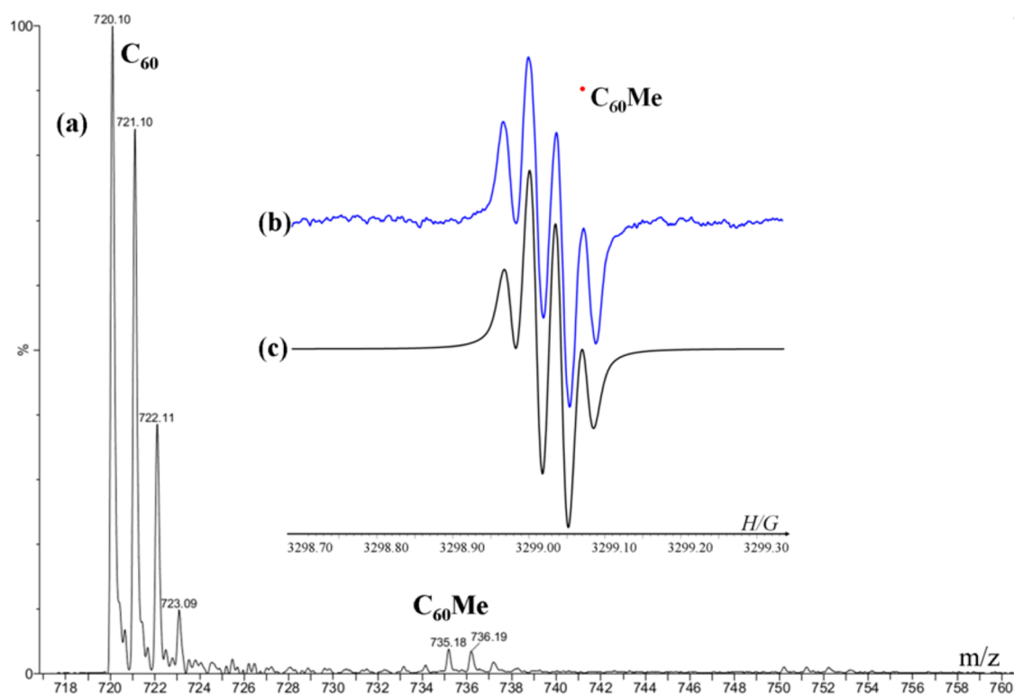
Figure 6. MALDI-TOF analysis of the sample prepared from complex 15 and MAO using fullerene as radical trapping agent. Catalyst added in a ratio of complex 15 :MAO 1:100; (a) MALDI-TOF spectrum of the reaction precipitate; (b) ESR spectrum of the reaction mixture at high resolution ( a_H(3H) = 0.035 G) under visible light irradiation ( \lambda > 550 nm); (c) simulated spectrum of \cdot C_{60}Me .
