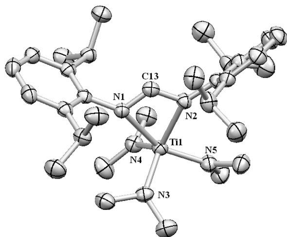
Figure 2. Mercury presentation of the molecular structure of complex 8 (50% probability ellipsoids). Hydrogen atoms are omitted for clarity. Representative bond lengths (Å) and angles (deg): Ti(1)–N(1) = 2.2926(13); Ti(1)–N(2) = 2.1847(13); Ti(1)–N(3) = 1.9087(15); Ti(1)–N(4) = 1.9002(14); Ti(1)–N(5) = 1.9130(14); C(13)–N(1) = 1.310(2); C(13)–N(2) = 1.328(2) Å; N(2)–Ti(1)–N(1) = 60.20(5); N(2)–Ti(1)–N(3) = 123.28(6); N(3)–Ti(1)–N(5) = 98.64(6); N(4)–Ti(1)–N(3) = 106.77(6); N(1)–C(13)–N(2) = 116.87(15); N(2)–Ti(1)–N(1)–C(13) = 3.69°.
