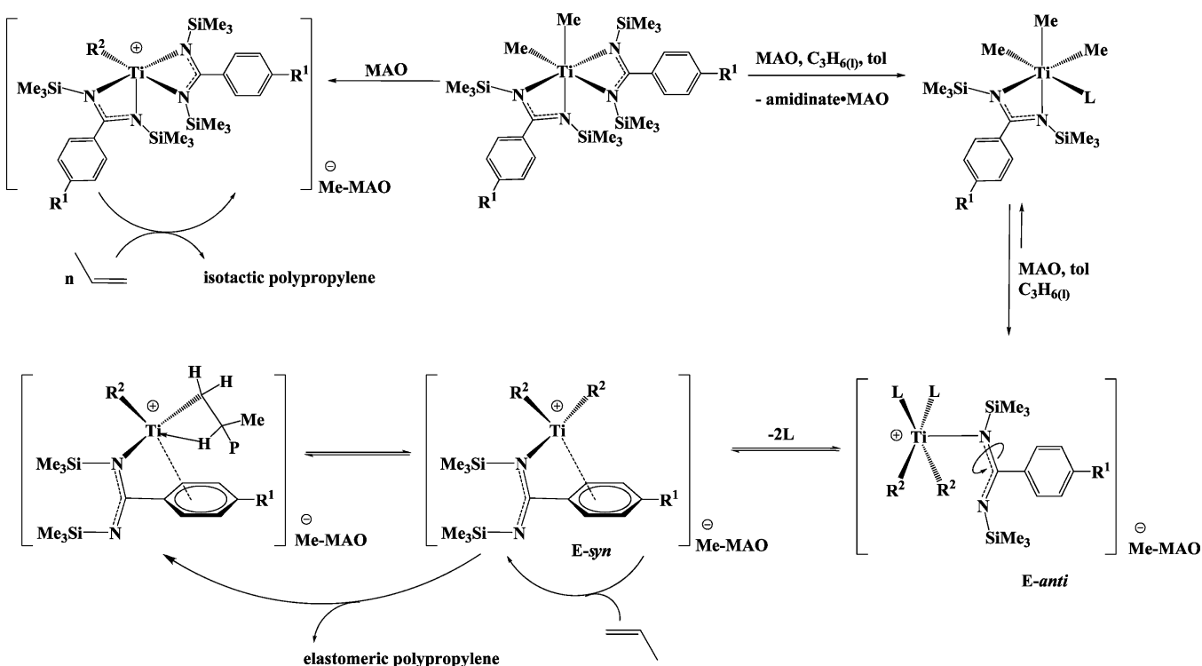
Scheme 1. Plausible Mechanism for the Formation of a Mixture of Isotactic and Elastomeric Polypropylene by Titanium Bis(amidinate) Complexes
