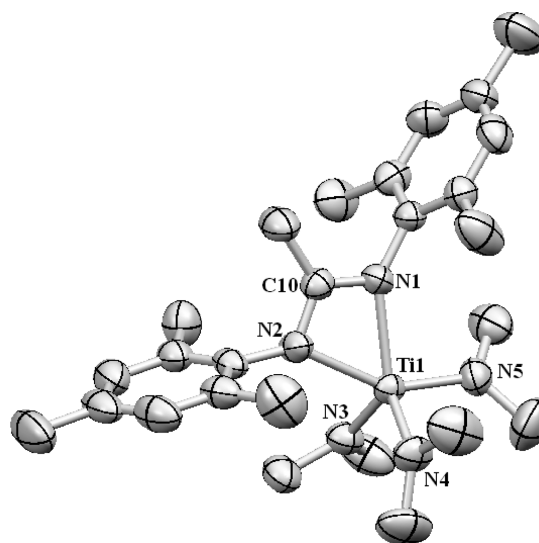
Figure 4. Mercury presentation of the molecular structure of complex 10 (50% probability ellipsoids). Hydrogen atoms are omitted for clarity. Representative bond lengths (Å) and angles (deg): Ti(1)–N(1) = 2.181(4); Ti(1)–N(2) = 2.232(4); Ti(1)–N(3) = 1.904(4); Ti(1)–N(4) = 1.901(4); Ti(1)–N(5) = 1.939(4); C(10)–N(1) = 1.327(6); C(10)–N(2) = 1.317(6) Å; N(2)–Ti(1)–N(1) = 59.92(14); N(1)–Ti(1)–N(5) = 91.63(16); N(5)–Ti(1)–N(4) = 99.73(19); N(1)–Ti(1)–N(4) = 128.07(16); N(1)–C(10)–N(2) = 113.0(4); N(2)–Ti(1)–N(1)–C(10) = 0.2(2)°.
