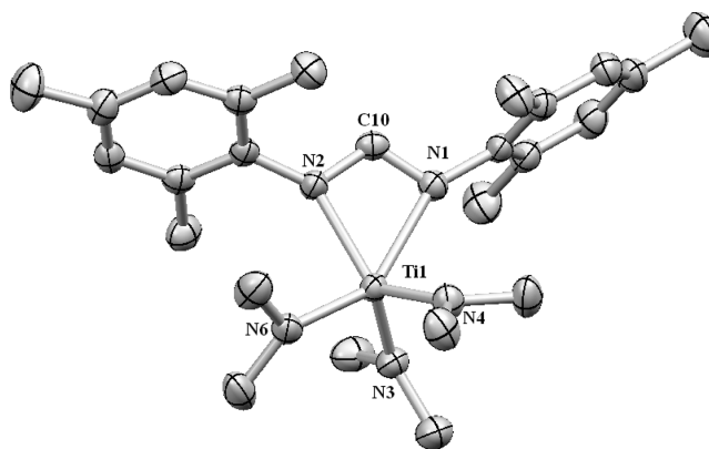
Figure 3. Mercury presentation of the molecular structure of complex 9 (50% probability ellipsoids). Hydrogen atoms are omitted for clarity. Representative bond lengths (Å) and angles (deg): Ti(1)–N(1) = 2.3087(12); Ti(1)–N(2) = 2.1372(12); Ti(1)–N(3) = 1.8838(13); Ti(1)–N(4) = 1.9115(13); Ti(1)–N(6) = 1.9197(13); C(10)–N(1) = 1.3055(19); C(10)–N(2) = 1.3251(19) Å; N(2)–Ti(1)–N(1) = 59.56(4); N(2)–Ti(1)–N(5) = 89.51(5); N(2)–Ti(1)–N(4) = 124.29(5); N(1)–C(10)–N(2) = 114.55(13); N(2)–Ti(1)–N(1)–C(13) = 5.74°.
