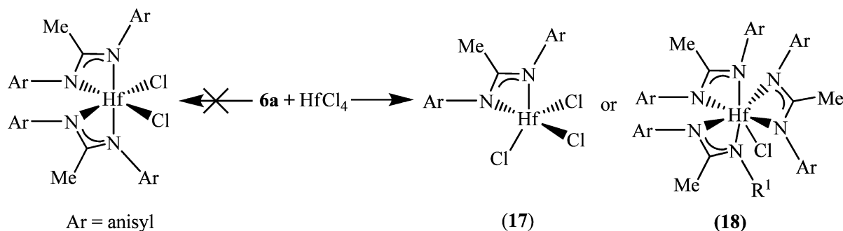
Scheme 3. Reaction of 6a with HfCl 4 Showing the Formation of Mono- or Tris(amidinate) Complexes
