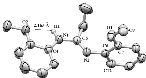
Figure 1. Mercury presentation of the molecular structure of ligand 7 showing the hydrogen bond interaction between the OMe moiety and the N–H amidine group (50% probability ellipsoids). Hydrogen atoms (besides the amidine N–H) were removed for clarity. Representative bond lengths (Å) and angles (deg): C(5)–N(1) = 1.3743(16); C(5)–N(2) = 1.2731(16); C(4)–N(1) = 1.4023(17); C(6)–N(2) = 1.4099(16); C(7)–O(1) = 1.3681(16); C(8)–O(1) = 1.4206(18) Å; N(2)–C(5)–N(1) = 120.66(12); C(7)–O(1)–C(8) = 117.70(11); C(5)–N(2)–C(6)–C(12) = 87.74°.
